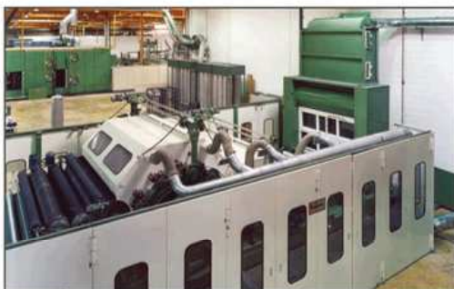
Compact TA-4/10/14-DLL-D 棉胎生产的梳棉 Card for the production of wadding
